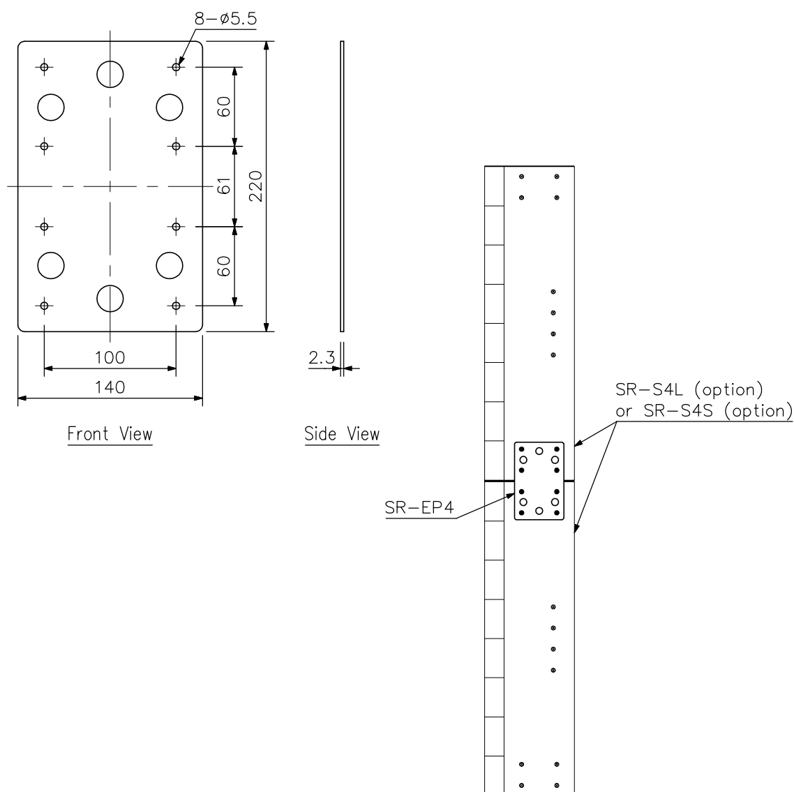
Mounting example (scale: 1/15)
