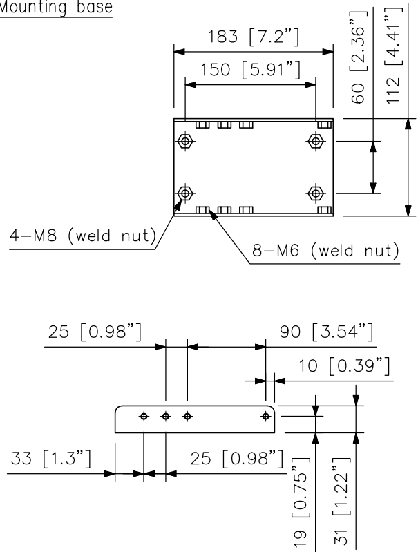
Mounting base
