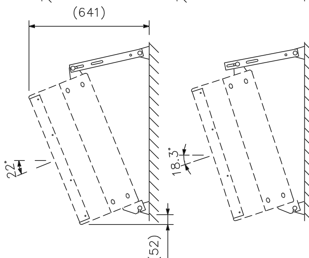
ES-0871 mounting example (scale: 1/20)
