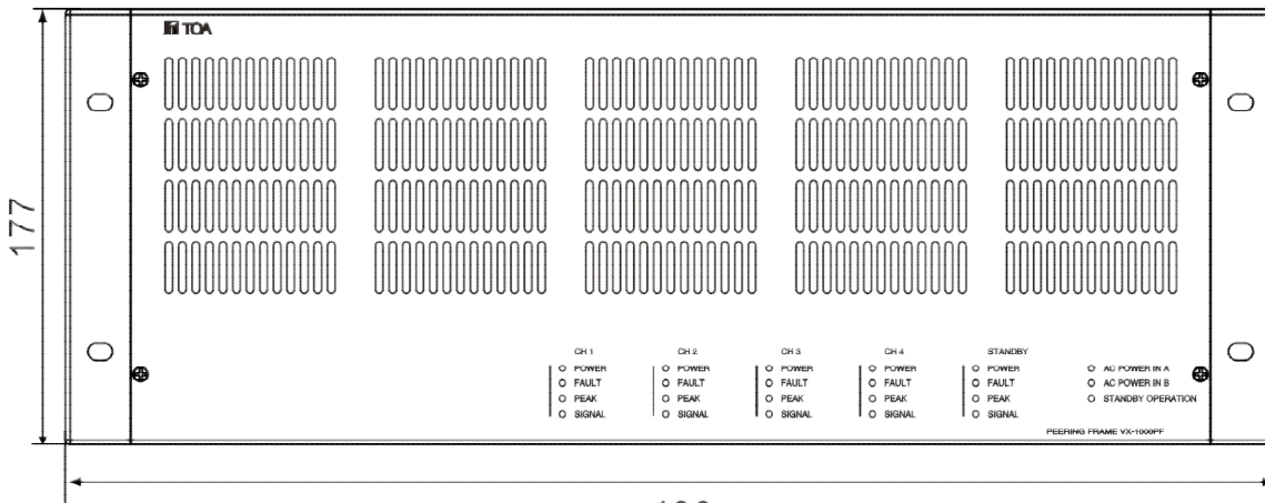
493 Front view
