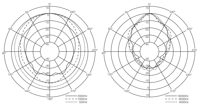
Polar Response - Horizontal -
