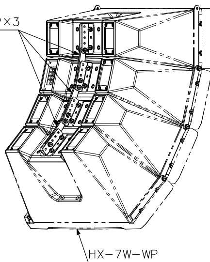
Mounting example (scale: 1/10)
